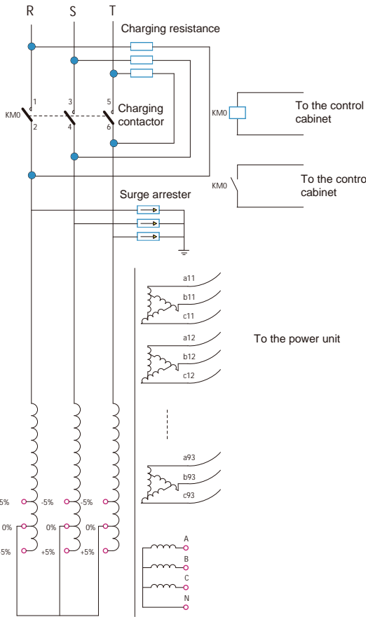
Anti-surge circuit diagram for a system
