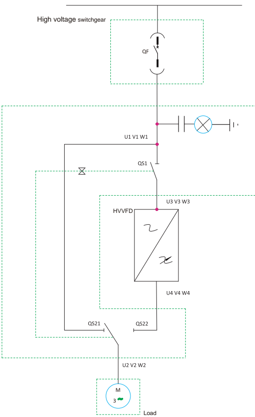
Manual one-drive-one bypass
