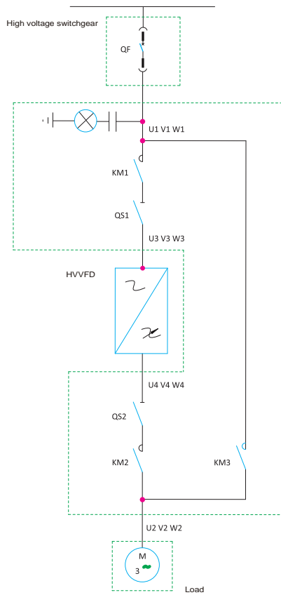
Automatic one-drive-one bypass
