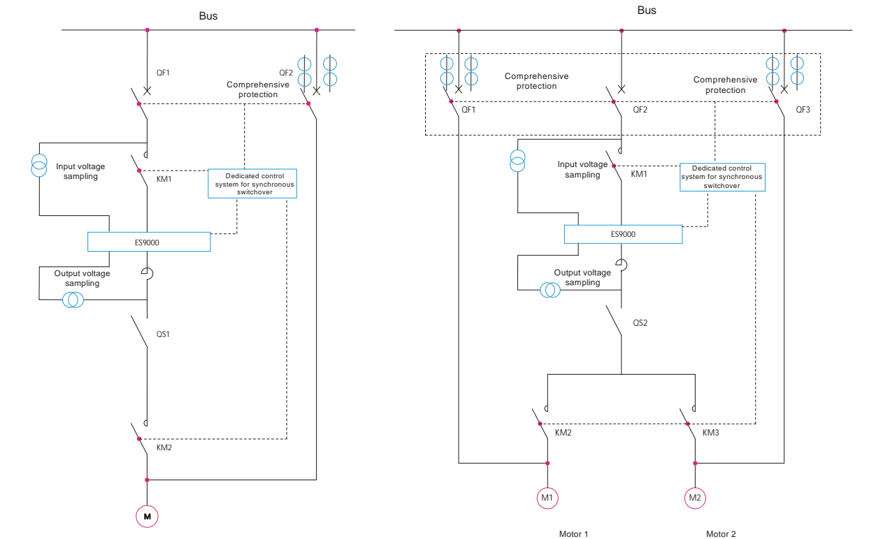
One-drive-one synchronous switchover softstart MVVFD
